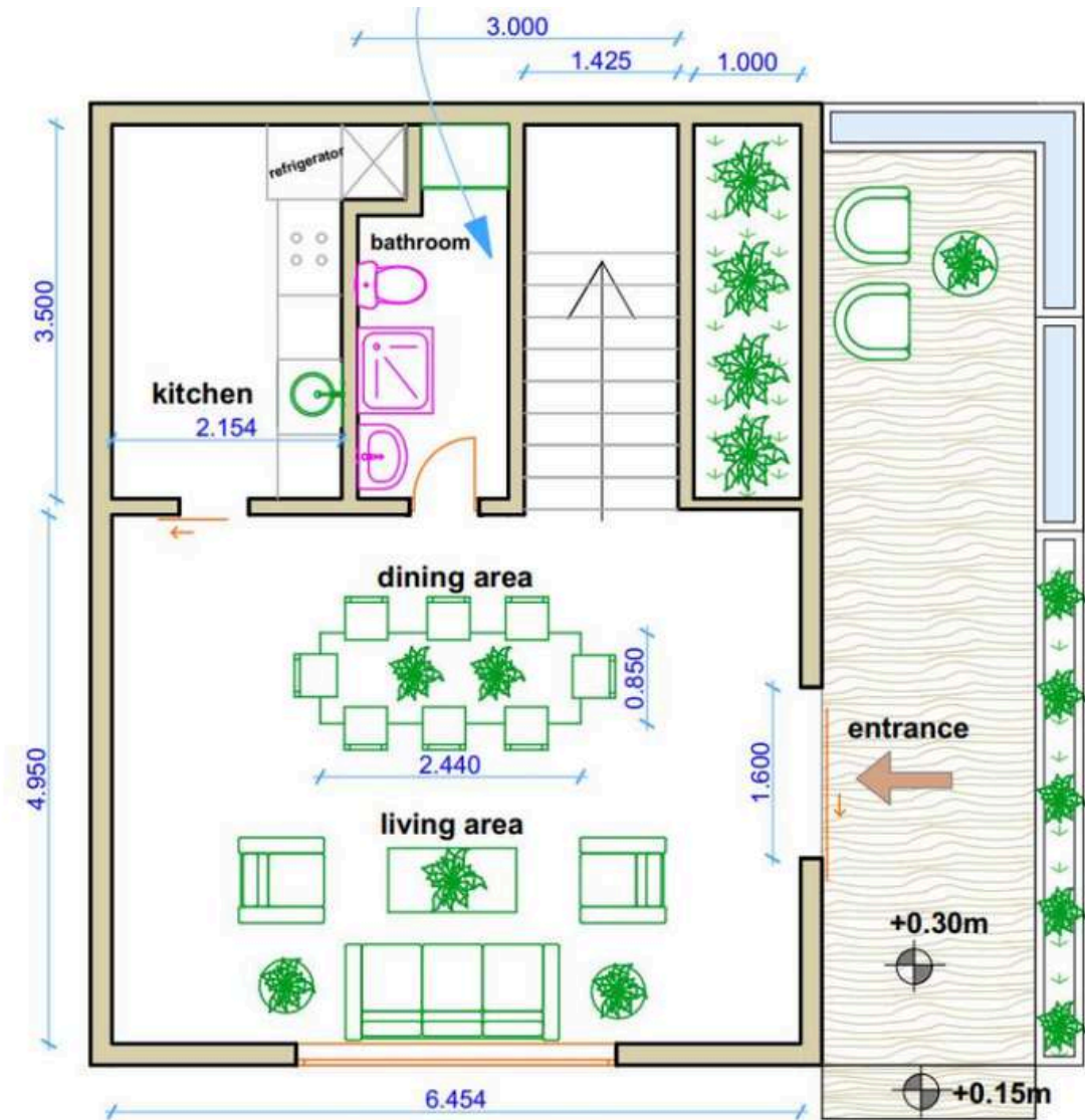
GROUND FLOOR
