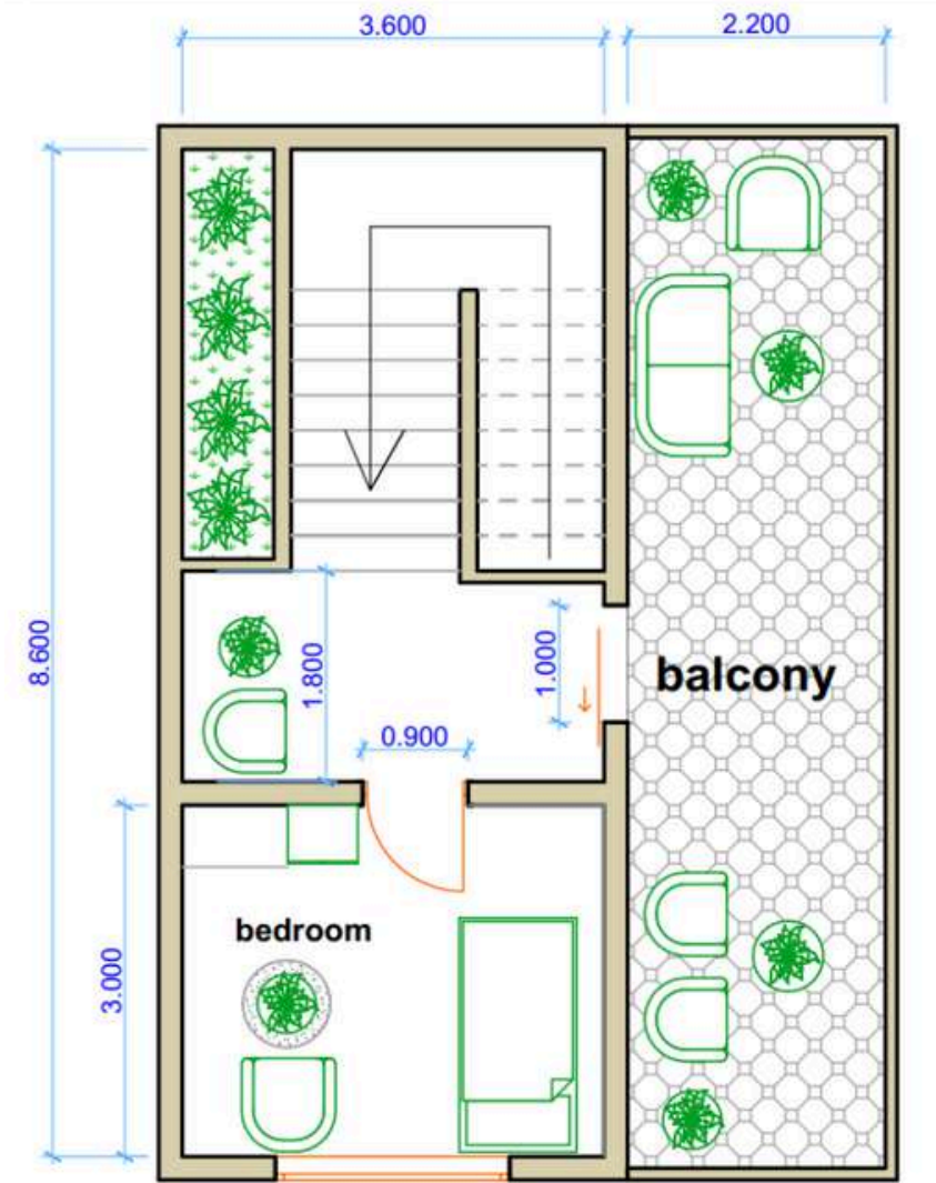
FIRST FLOOR
